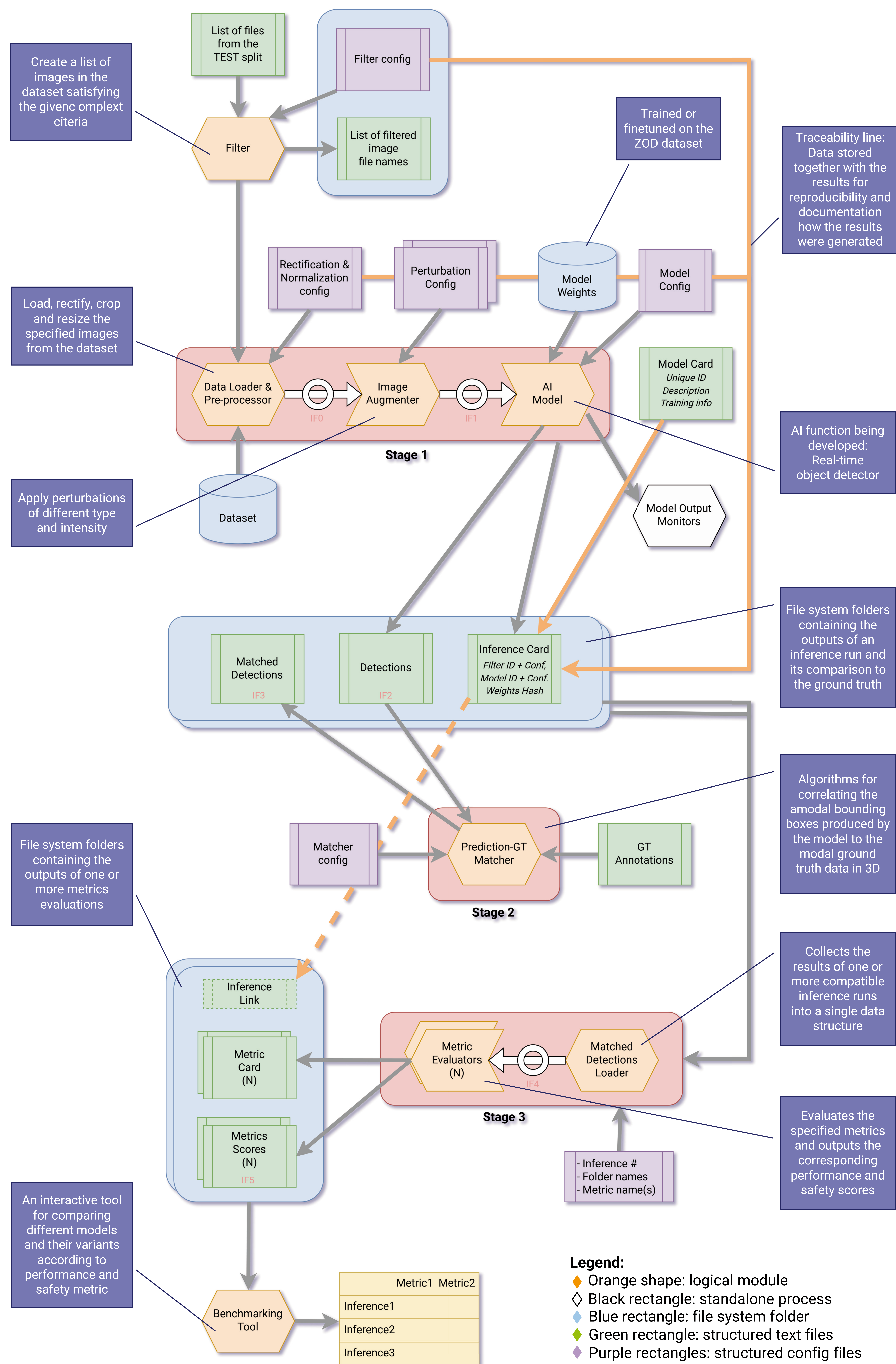
Figure 2: Data and traceability flow in the SRP metrics evaluation pipeline
